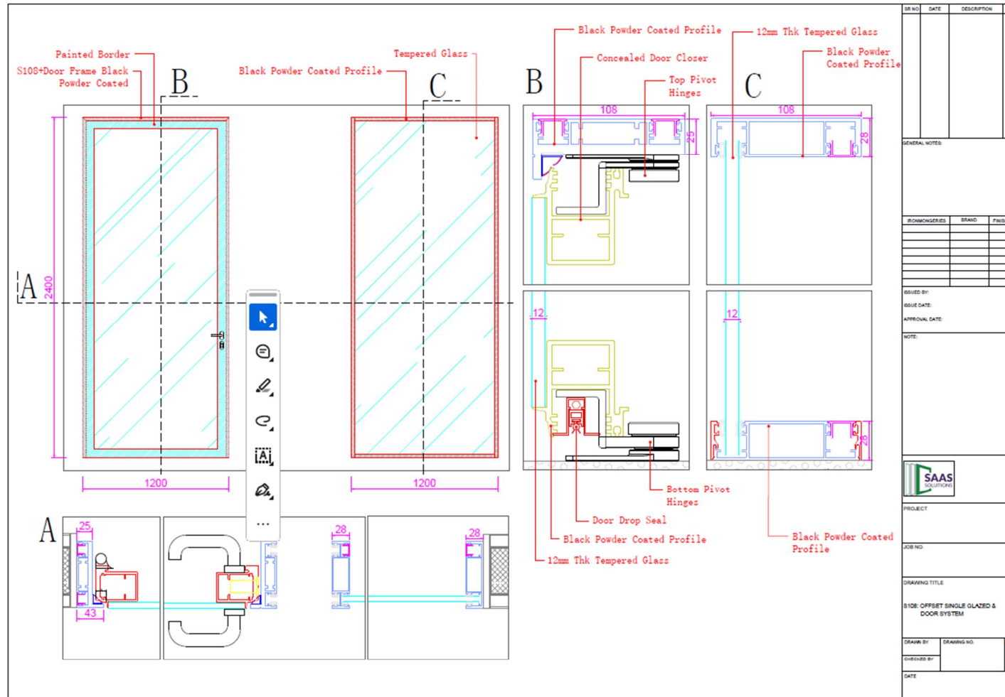
Appendix : Technical drawing of the "S108 Offset Single Glazed" partition system with 12mm thick tempered glass
