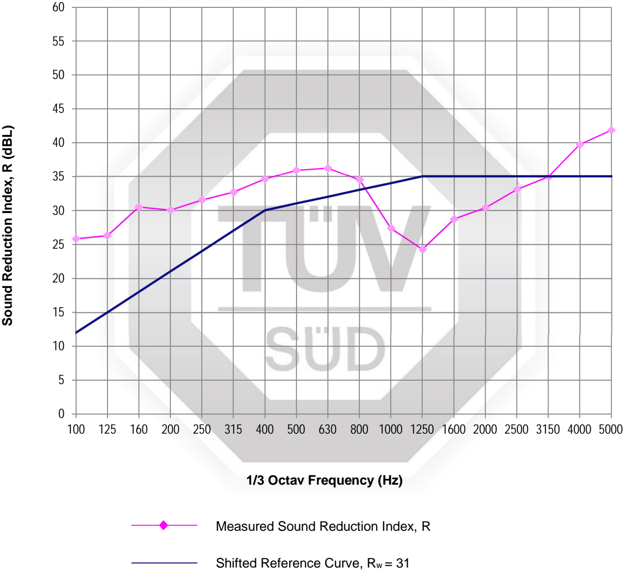
Figure 1: Sound Insulation Performance of “S-68 Single Glazed” Partition System with 12mm thick tempered glass (R w 31)
